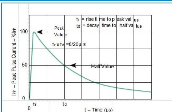
Figure 8 - Pulse Waveform
