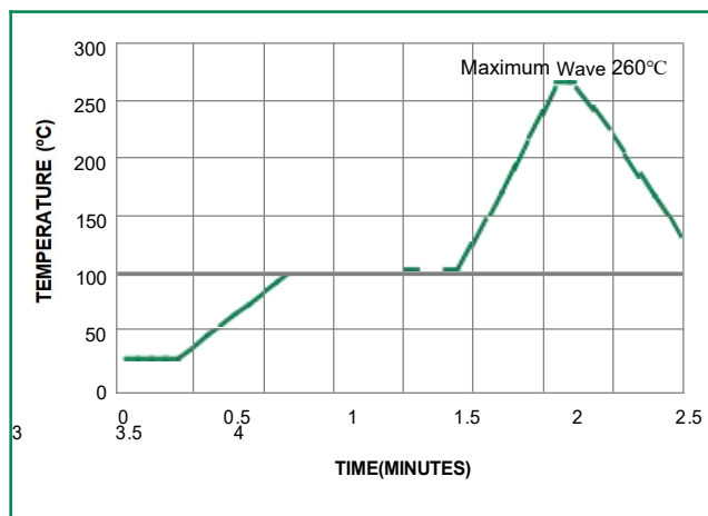
Figure 2 - Lead-free Profile
